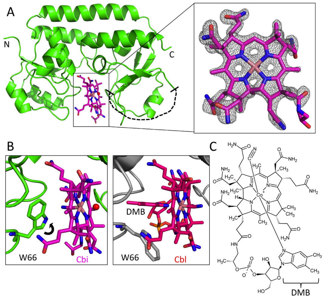
Figure 2. Crystal structure of Cbi-bound BtuF. (A) Cbi-bound BtuF model (PDB ID 5M29). BtuF is depicted in green cartoon and cyano-aquo-cobinamide is shown in stick representation (carbon, magenta; oxygen, red; nitrogen, blue; cobalt, light brown). The N- and C-termini of BtuF are indicated as N and C, respectively. After initial rounds of refinement with omission of the ligand in the model, unambiguous electron density for Cbi was displayed in the Fo-Fc map contoured at \pm 3.0\sigma (box to the right and viewed from C-lobe). The disordered amino acid residue stretch (217 to 232) is indicated with a dashed black line. (B) Comparison of the substrate binding sites of Cbi-bound BtuF (left box) and Cbl-bound BtuF (right box, PDB ID 1N4A). In Cbi-bound BtuF residue W66 adopts a new rotamer (black arrow) facing the inside of the substrate binding site and filling the space occupied by DMB in Cbl-bound BtuF. The two axial ligands of Cbi, a cyanide and a water molecule, are shown as stick and red sphere, respectively. For Cbi-bound BtuF the same coloring was used as in panel A. Cbl-bound BtuF is illustrated as gray cartoon for the protein part and stick representation for Cbl (carbon, red; oxygen, red; nitrogen, blue; cobalt, light brown; phosphate, yellow). Both substrate binding sites are shown from the front view similar to panel A. (C) Chemical structure of the bigger substrate Cbl illustrating the additional 5,6-dimethylbenzimidazole (DMB) moiety and sugar-phosphate linker, which are absent in the smaller substrate Cbi. The two axial ligands DMB and cyanide are in the \alpha - and \beta -position, respectively, and coordinated by the central Co atom.
