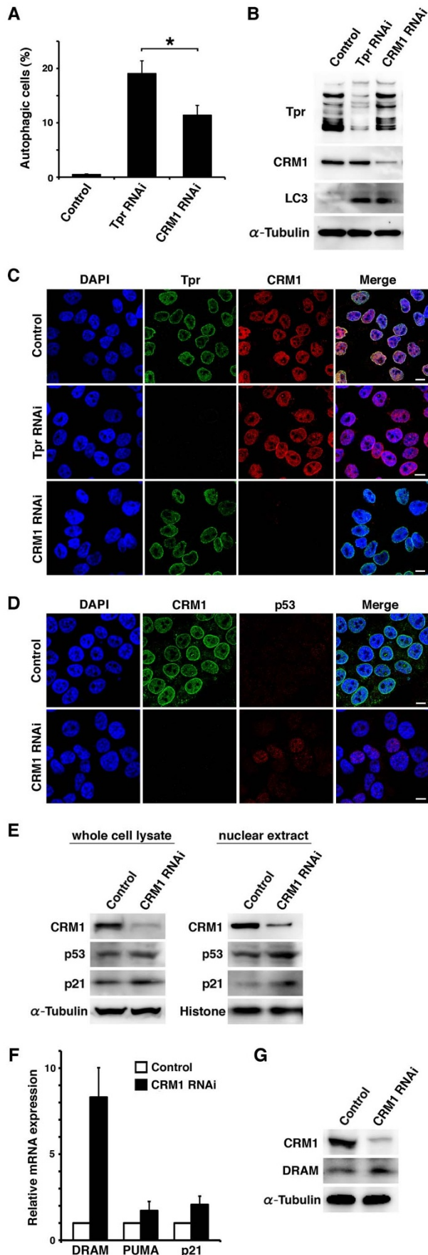
Figure 6 | CRM1 depletion also induces autophagy, but weaker than Tpr depletion. (A) Quantification of acridine orange staining in Tpr or CRM1 siRNA transfected HeLa cells. HeLa cells were transfected with control, Tpr or CRM1 siRNA for 72 h, and were analyzed by acridine orange staining to determine the ratio of autophagy. At least 500 cells in each experiment were examined under a fluorescence microscope and the percentage of acridine orange staining cells was calculated. The data are presented as the means \pm S.D. for three different experiments. *, P < 0.05 . (B) HeLa cells transfected with control, Tpr, or CRM1 siRNA were analyzed by immunoblot for Tpr, CRM1, and LC3 expression. Representative results of three different experiments are shown. (C) HeLa cells were transfected with control, Tpr, or CRM1 siRNA for 72 h, and then Tpr and CRM1 were visualized by immunofluorescence following nuclear DAPI staining. Scale bars, 10 \mu m. (D) HeLa cells were transfected with control or CRM1 siRNA for 72 h, and then CRM1 and p53 were visualized by immunofluorescence following nuclear DAPI staining. Scale bars, 10 \mu m. (E) HeLa cells transfected with control or CRM1 siRNA were analyzed by immunoblot for CRM1, p53 and p21 expression. Representative results of three different experiments are shown. (F) HeLa cells transfected with control or CRM1 siRNA for 72 h and mRNA levels were assayed by quantitative PCR. The data are presented as the means \pm S.D. for triplicate determinations. bars, SD. (G) HeLa cells transfected with control or CRM1 siRNA were analyzed by immunoblot for CRM1 and DRAM expression. Representative results of three different experiments are shown.
