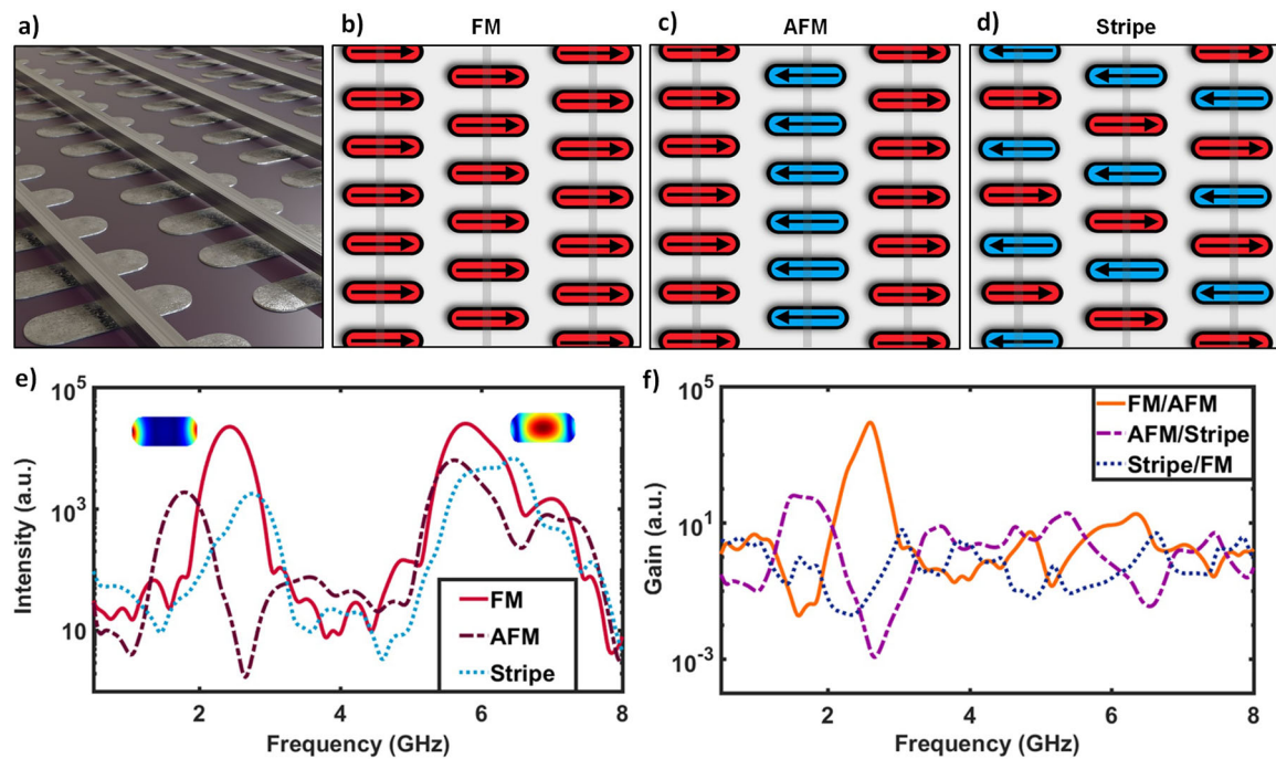
Fig. 4 Two-dimension magnonic crystal. a Schematic of the 2D magnonic crystal incorporating control nanowires above each column of the nanomagnet array. b–d Schematics of the b FM, c AFM and d ‘stripe’ microstates illustrating magnetization directions of each nanoisland and control-nanowire positions. e Spin-wave spectra of ferromagnetic (FM), antiferromagnetic (AFM) and ‘stripe’ microstates on a 4 \times 6 nanoisland magnonic crystal. Each state shows two main resonances, an edge-localized mode (1–3 GHz) and a centrally localized mode (5–8 GHz). Spatial magnon power maps for each mode are displayed next to peaks. f Spin-wave amplitude gain achieved by transitioning between microstates, i.e., moving from FM to AFM state (solid orange line).
