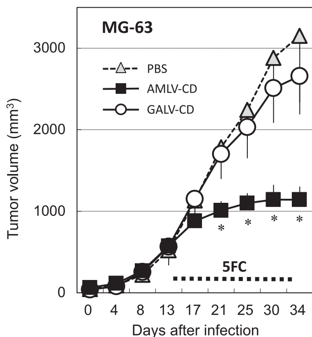
Fig. 4 In vivo antitumor effect of AMLV vs. GALV-mediated prodrug activator gene therapy in a subcutaneous xenograft model of human osteosarcoma cells. MG-63 tumors were grown subcutaneously in nude mice to 5–6 mm in diameter, then injected intratumorally with 1 \times 10^4 TU (50 \mu L) of either AMLV-CD or GALV-CD, or PBS vehicle control on Day 0, followed by intraperitoneal administration of 5FC (500 mg/kg/day) three times weekly from Day 14 to Day 34 ( n = 10 per group). Tumor volumes were measured twice weekly, and data shown are averages—(PBS and GALV-CD) or +(AMLV-CD) SD from experiments. * P < 0.01 (AMLV-CD vs. GALV-CD)
