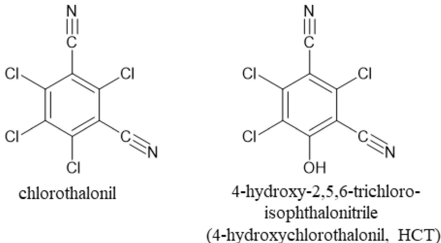
Fig. 1 Chemical structures of chlorothalonil and 4-hydroxychlorothalonil (HCT).
