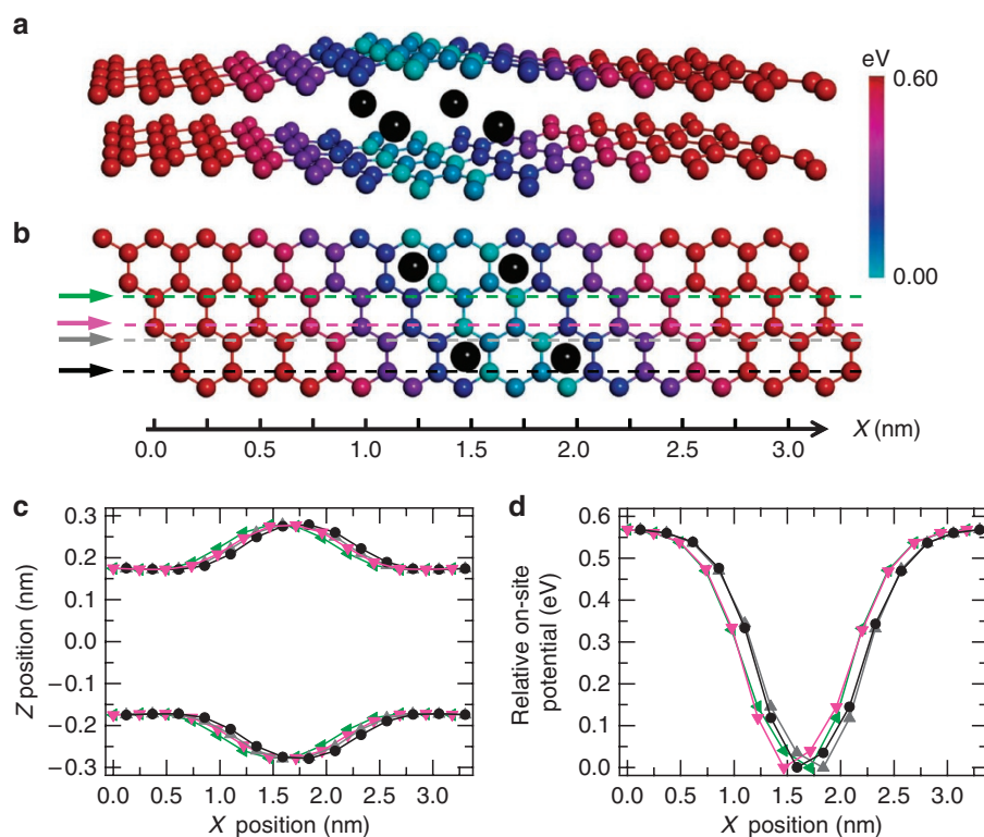
Figure 3 | Structure and on-site potential of partially potassium-intercalated bilayer graphene calculated by DFT. (a,b) A perspective side view and an orthogonal top view, respectively. The colour indicates the relative on-site potential of each carbon atom. The minimum energy is set as 0 eV. (c,d) The Z positions and relative on-site potentials of the carbon atoms along the dashed lines in b with the same colours as a function of the X position, respectively.
