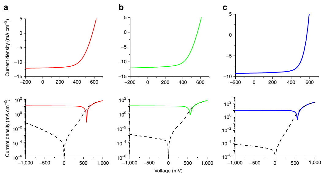
Figure 3 | J-V characteristics. (a) Linear-linear (top) and log-linear (bottom) J - V characteristics of an optimized ultrathin OPV device on 1.4\mu\text{m} PET substrate. The device performance metrics are V_{OC} = 580\text{ mV} , J_{SC} = 11.9\text{ mA cm}^{-2} , FF = 61% and \eta = 4.2\% . Solid lines are measured under one sun illumination and dashed lines in the dark (also in b,c). (b) Device performance of reference device, using the same materials but constructed directly on glass substrates without PET. The device performance metrics are V_{OC} = 565\text{ mV} , J_{SC} = 11.9\text{ mA cm}^{-2} , FF = 61% and \eta = 4.1\% . Comparing the J - V curves of a and b, nearly identical behaviour is observed. The V_{OC} of this particular device is slightly lower, but overall the performance of the glass and PET-based solar cells is indistinguishable. (c) Ultrathin OPV devices on PET foil with underlying silver grid can attain FF up to 71% (top) and dark diode rectification of up to 6 orders of magnitude at \pm 1\text{ V} (bottom). However, they typically show lower J_{SC} due to shading from the silver grid.
