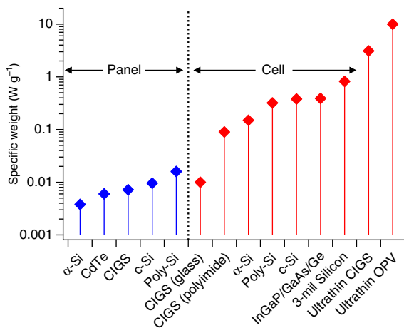
Figure 7 | Comparing solar cell technologies. Specific weight of various photovoltaic technologies for complete modules (left) and individual cells (right). Module data are taken from manufacturer-specified efficiency and weight of commercially available panels and should be representative: Kaneka 12V 55W PV Module, First Solar F5272, Sunforce 70W Pro Series, Bosch Solar Module c-Si M60 and Kyocera KD245Gx-LPB. Cell data were taken from published academic results. In many cases, the cell weight was not published and so was estimated from published layer thicknesses and known material densities, assuming 2% areal coverage for metal grid contacts 17,18,23–27 . For a direct comparison of cell efficiency, please see Green et al. 6 .
