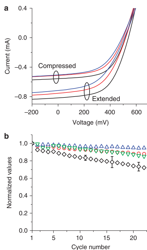
Figure 6 | Resilience to cyclic compression-stretching. Device performance during 22 consecutive compression-stretch cycles to 50% compression. (a) The I-V characteristics are shown at 1 (black), 11 (red) and 22 (blue) cycles for both the fully extended and 50% (quasi-linear) compressed states. (b) Device performance metrics plotted at each of the 22 cycles for the fully extended state. Green downward triangles represent FF, blue upward triangles V_{OC} , red circles I_{SC} and black diamonds power. All parameters are normalized to their initial value. Upon cycling, a reduction of the FF and I_{SC} is observed. The origin of these losses is unknown, but is certainly in part owing to the experimental apparatus and loss of contact. The overall efficiency is shown to be 73% of its original value after 22 repeated cycles. Multiple separate devices were subjected to cyclic testing. For the sake of clarity, error bars are indicated only for the power metric for selected data points, as this is the primary metric for device characterization.
