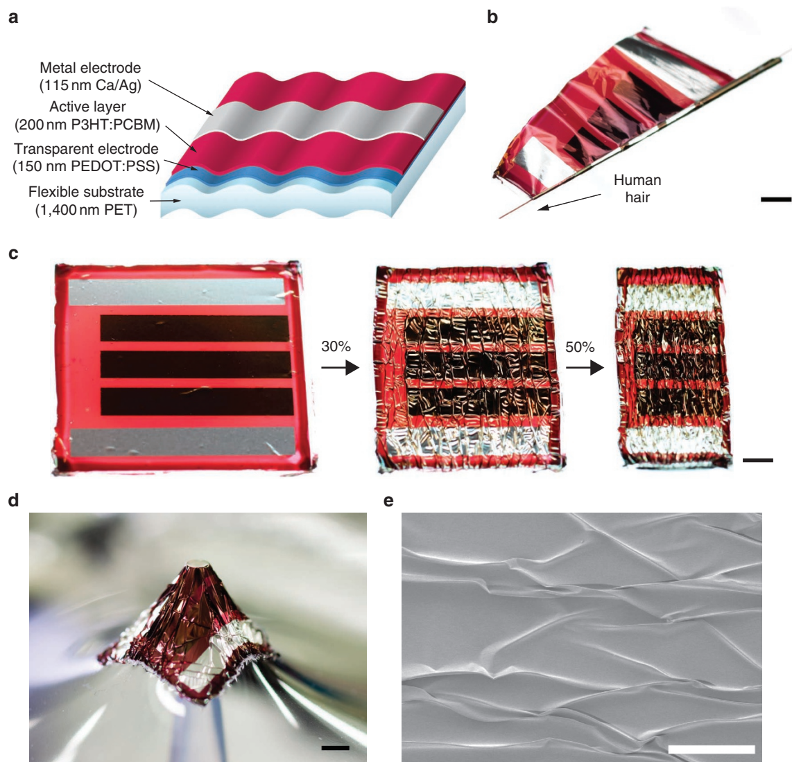
Figure 1 | Sub-2- \mu\text{m} -thick organic solar cells. (a) Scheme of the ultra-light and flexible organic solar cell. The layer thicknesses are drawn to scale. (b) Extreme bending flexibility demonstrated by wrapping a solar cell around a 35- \mu\text{m} -radius human hair. Scale bar (also in c,d) 2 mm. (c) Stretchable solar cells made by attaching the ultrathin solar cell to a pre-stretched elastomer. They are shown flat (left) and at 30% (middle) and 50% (right) quasi-linear compression. (d) The device attached to the elastomeric support, under three-dimensional deformation by pressure from a 1.5 mm-diameter plastic tube. (e) SEM image of the PET surface of the solar cell in compressed state. The radius of curvature for the shown wrinkles is estimated to be on the order of 10 \mu\text{m} . Scale bar 500 \mu\text{m} .
