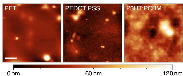
Figure 2 | AFM images of the individual device layers. AFM topographical image of the 1.4\mu\text{m} Mylar CW02 substrate foil on glass/PDMS support (left). The RMS roughness is \approx 12\text{ nm} with a maximum peak-to-peak distance of 162\text{ nm} . Image of the PEDOT:PSS transparent electrode on PET (centre). RMS roughness is \approx 12\text{ nm} and the maximum peak-to-peak distance is 116\text{ nm} . Image of the P3HT:PCBM active layer atop the transparent electrode (right). The RMS roughness is \approx 16\text{ nm} and the maximum peak-to-peak distance is 130\text{ nm} . Scale bar 1\mu\text{m} .
