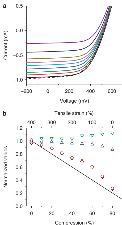
Figure 4 | Extreme mechanical deformation. (a) I-V curves during compression on pre-stretched elastomer. The solid black line represents 0% and the purple line represents 80% compression with the intermediate steps of 10% distributed between accordingly. The dashed black line represents the device after re-stretching from 80% compression to its initial flat state. (b) Measured device parameters 0–80% compression, which correspond to 400–0% tensile strain or five times change in size. Green downward triangles represent FF, blue upward triangles V_{OC} , red circles I_{SC} and black diamonds power. All parameters are normalized to their pre-compression value. The I_{SC} and correspondingly the total maximum power of the solar cell decrease, but maintain higher values than would be expected with the corresponding decrease of device area, represented by the black line. Upon re-stretching the device to its original size, the values are nearly identical to the pre-compression state. The symbol size is chosen to represent the reproducibility of the experiment, as indicated by error bars for selected data points for the power metric.
