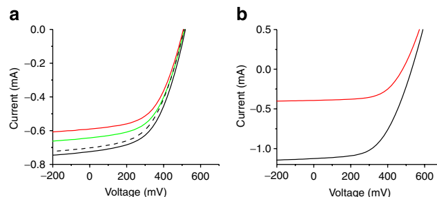
Figure 5 | Biaxial compression. (a) The device performance under reversible biaxial compression of 0% (black solid line), roughly 10% (green solid line) and roughly 20% (red solid line). Upon re-stretching to near flat conditions, the device shows comparable performance (black dashed line). (b) Device performance under very high biaxial compression of more than 50% (red solid line) compared with 0% flat state (black solid line).
