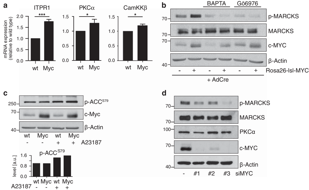
Figure 3. MYC selects for increased calcium signalling. (a) Total RNA isolated from WT or Rosa26-lsl-MYC MEFs harvested 24 h after infection with Adeno-CRE was analysed by Q-PCR for expression of the indicated transcripts. Mean and s.d. from biological triplicates shown. Statistical significance was determined by two-tailed unpaired T -tests. (b) Immunoblot from Adeno-CRE-infected WT or Rosa26-lsl-MYC MEFs as per (a) probed for expression and phosphorylation of the PKC substrate MARCKS. Where indicated, MEFs were treated with BAPTA (10 \mu M for 3 h) or Gö6976 (1 \mu M for 3 h) prior to lysis. (c) Lysates from WT and MYC-transformed MEFs, treated as indicated with 10 \mu M A23187 (10 min), probed with the indicated antibodies. Densitometry analysis shows normalized levels of p-ACC S79 from three immunoblots. (d) Immunoblot from HeLa cells upon depletion of MYC using three independent siRNAs versus non-targeting control (-), probed for p-MARCKS S159/163 . All images are representative of at least three independent experiments, except (d) where N = 2.
