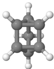
QC ( r_{cc}=1.51 \text{ \AA} )
